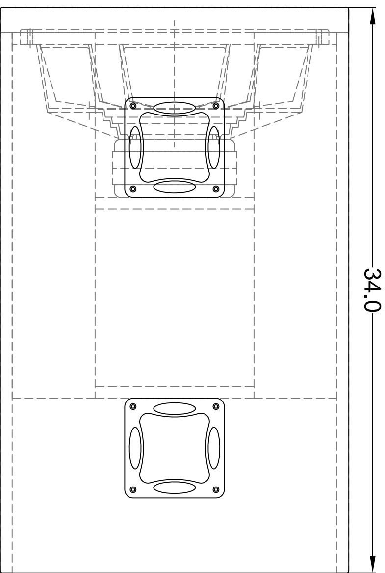
S182A - single 18 vented cabinet 28Hz tune
